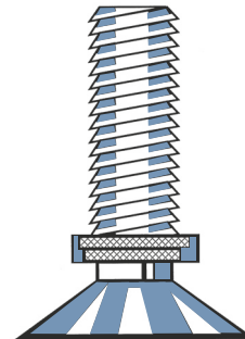
Illustration 17 : Valve Schrader
