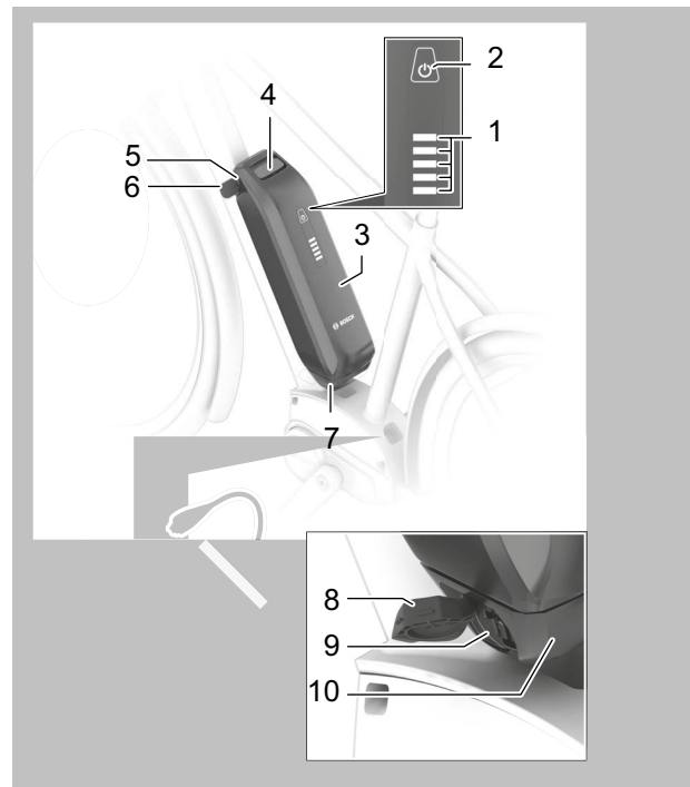
Figur 35: Detaljer for PowerPack
